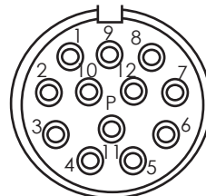
Motor Side: SFMB12MRSN000 PIN Arrangement
