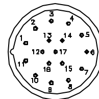
INTERCONNECTOR SIZE 1 17 PIN
