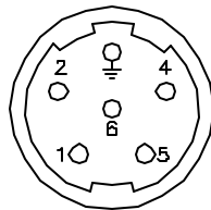
INTERCONNECTOR SIZE 1 6 PIN
