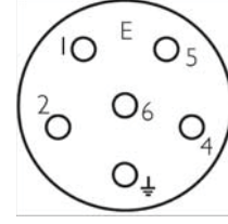
Mating Connector: LPRA06BFRDN170 PIN Arrangement
