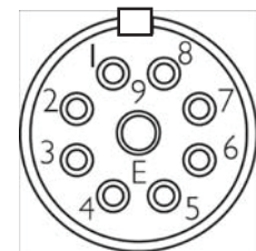
Cable Side: SPNA09FFROR169 PIN Arrangement
